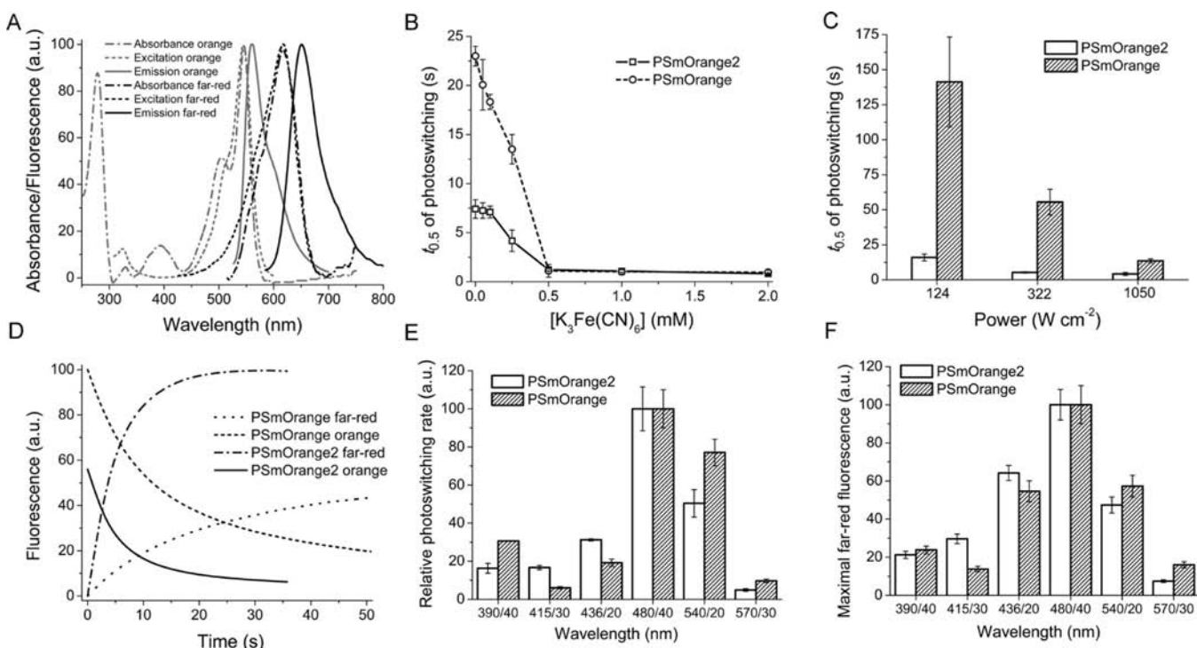
Figure 2. Properties of the purified PSmOrange2 protein. (A) Absorbance, excitation and emission spectra of PSmOrange2 before and after photoswitching with 489 nm LED array. (B) Photoswitching half-times ( t_{0.5} ) for PSmOrange2 and PSmOrange at indicated K_3Fe(CN)_6 concentrations and 1050 mW\ cm^{-2} light power density. (C) Photoswitching half-times ( t_{0.5} ) for PSmOrange2 and PSmOrange at indicated light power densities and 0.25 mM of K_3Fe(CN)_6 . (D) Photoswitching kinetics for orange and far-red forms of PSmOrange and PSmOrange2. (E) Initial rates of photoswitching for PSmOrange and PSmOrange2 at indicated photoswitching wavelength bands normalized to 100% at 480/40 nm. (F) Maximal far-red fluorescence of PSmOrange2 and PSmOrange achieved at indicated photoswitching wavelength bands normalized to 100% at 480/40 nm. In panels B–D, the 480/40 nm wavelength band was used for photoswitching. In panels D–F, the 0.25 mM of K_3Fe(CN)_6 and 1050 mW\ cm^{-2} light power density were applied. The power densities were estimated at the sample. Error bars, SD.
