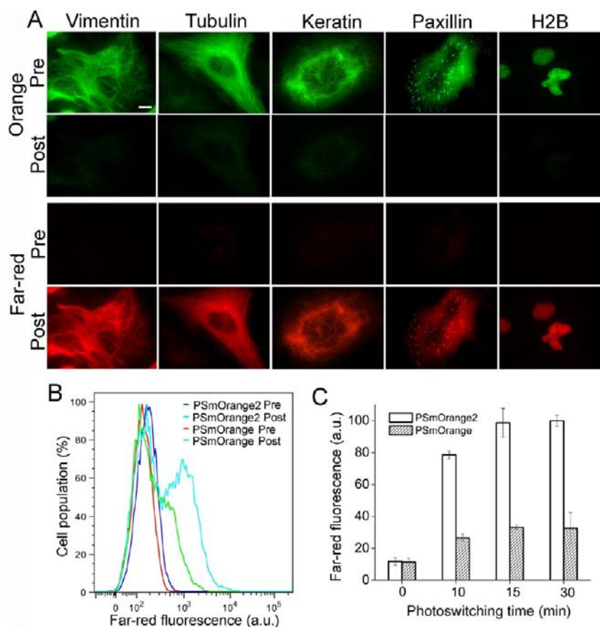
Figure 3. PSmOrange2 in live HeLa cells. (A) Cells expressing PSmOrange2 fusions with indicated proteins before (Pre) and after (Post) photoswitching. Images in orange (green) and far-red (red) channels are shown. Scale bar, 10 \mu\text{m} . (B) Flow cytometry analysis of cell populations expressing PSmOrange2 (blue and cyan lines) and PSmOrange (red and green lines) before (Pre) and after (Post) photoswitching. The 638 nm excitation laser and 660/20 nm emission filter were used. (C) Mean far-red fluorescence intensities of PSmOrange2 and PSmOrange expressing cells at indicated photoswitching times. The 647 nm excitation laser and 670/30 nm emission filter were used. Error bars, SD.
