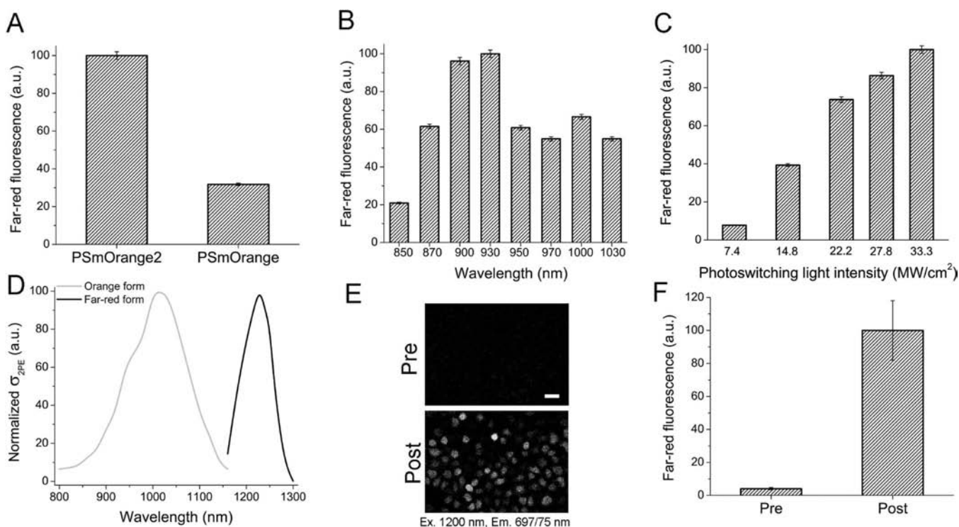
Figure 4. Properties of PSmOrange2 using two-photon excitation (2PE). (A) Far-red fluorescence intensity of PSmOrange2 and PSmOrange achieved by 2P photoswitching using 40 mW of 900 nm light scanning at 1 frame/s for 5 min. (B) Far-red fluorescence intensity achieved by 2P photoswitching using 90 mW of light at indicated wavelengths scanning at 1 frame/s for 30 s. (C) Far-red fluorescence intensity after 2P photoswitching with the indicated laser powers at 900 nm and scanning at 1 frame/s. The light intensity of 7.4, 14.7, 22.2, 27.8 and 33.3 MW/cm 2 at the sample corresponds to the laser power of 20, 40, 60, 75 and 90 mW, respectively. (D) Relative 2PE spectra ( \sigma_{2PE} ) of orange and photoswitched far-red PSmOrange2 forms. (E) 2P images of MTLn3 live cells expressing PSmOrange2 before (Pre) and after (Post) photoswitching using 90 mW of 2PE at 900 nm for 40 s. The 1200 nm 2PE and a 697/75 nm emission filter were used to generate and collect the fluorescence signal. Scale bar, 50 \mu m. (F) Mean far-red fluorescence intensities of PSmOrange2 expressing cells shown in panel E. Error bars, SD.
